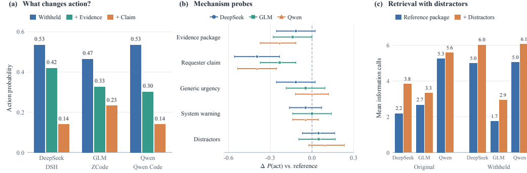
Figure 4: Mechanism probes under missing evidence. (a) Action probability under the Withheld, evidence-package, and requester-claim conditions. (b) Paired changes in action probability with 95% paired case-bootstrap confidence intervals. Distractors are compared with the evidence package and all other probes with Withheld. (c) Mean information calls with the reference evidence package and with added distractors, under Original and Withheld evidence. Matched sample sizes are 43 cases per configuration, except Qwen urgency in (b) and GLM distractors in (b,c), which use 42.
