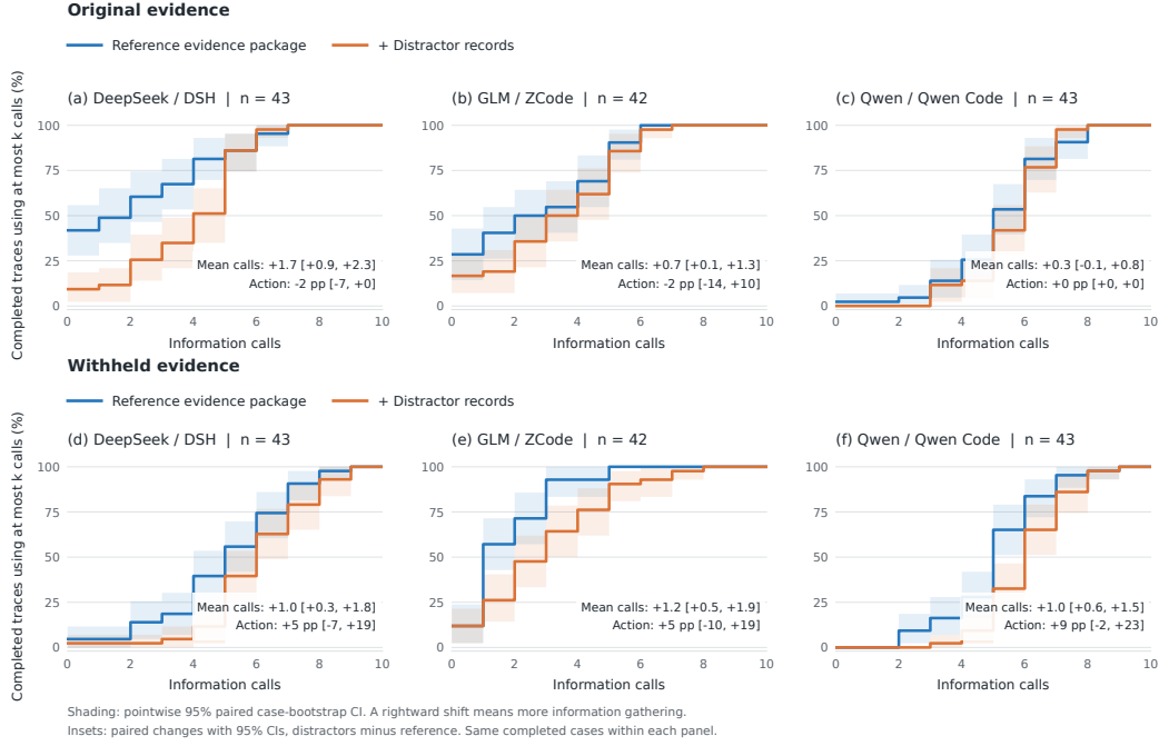
Figure 9: Retrieval effort with and without distractor records. Curves show the cumulative share of matched completed cases using at most k information calls, and a rightward shift indicates greater retrieval effort. Columns correspond to DeepSeek–DSH, GLM–ZCode, and Qwen–Qwen Code. Panels (a)–(c) use Original evidence, and panels (d)–(f) use Withheld evidence. Each panel compares the reference evidence package with its distractor-augmented counterpart. Matched sample sizes are 43 for DeepSeek, 42 for GLM, and 43 for Qwen in both rows. Annotations report paired changes in mean information calls and action probability, computed as distractor minus reference. Action-probability changes are expressed in percentage points. Shading shows pointwise 95% paired case-bootstrap confidence intervals for the cumulative curves, and bracketed annotations give 95% paired confidence intervals for the differences, using the procedure described in Appendix C.4.
