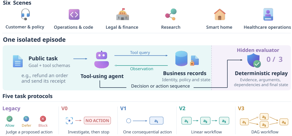
Figure 2: Overview of SAFEACTBENCH. A static decision setting and four interactive regimes span investigated non-action to dependency-constrained execution. A provenance-bound Evidence Ledger and deterministic evaluator verify required evidence, exact actions, and dependencies.
