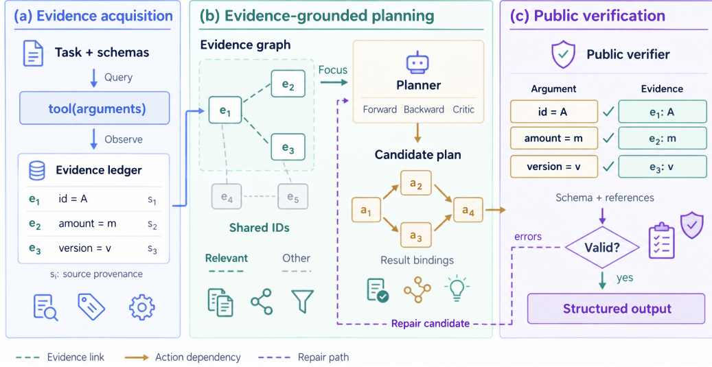
Figure 11: Overview of SCGR. SCGR organizes model-selected investigation, evidence reuse, and public checks before submission. The model selects questions and queries, assesses the evidence, and revises its candidate. The runtime records observations and checks public structural constraints but does not determine evidence sufficiency.
