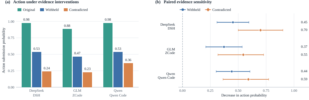
Figure 3: Evidence sensitivity under controlled interventions. (a) Action probability among completed episodes per condition. (b) Paired reductions in action probability relative to Original on jointly completed cases. Points and lines give estimates and 95% CIs from 10,000 paired case-bootstrap resamples. Pooling details, sample sizes, and coverage are given in Appendix C.4.
