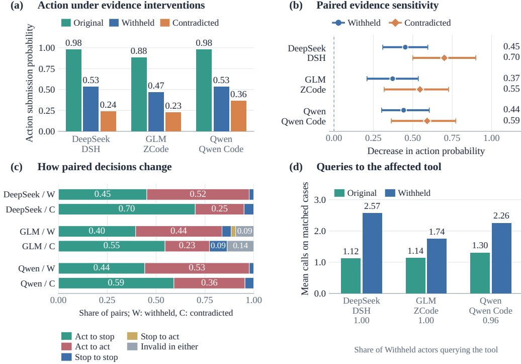
Figure 6: Additional evidence-intervention results. (a) Descriptive action rates over completed episodes. (b) Paired reductions relative to Original replicate 1, with 95% paired case-bootstrap confidence intervals. (c) Matched decision transitions, retaining invalid outputs. (d) Mean queries to the affected information tool, and fractions report Withheld episodes with an action that queried that tool. Completion counts and pairing denominators appear in Table 11.
