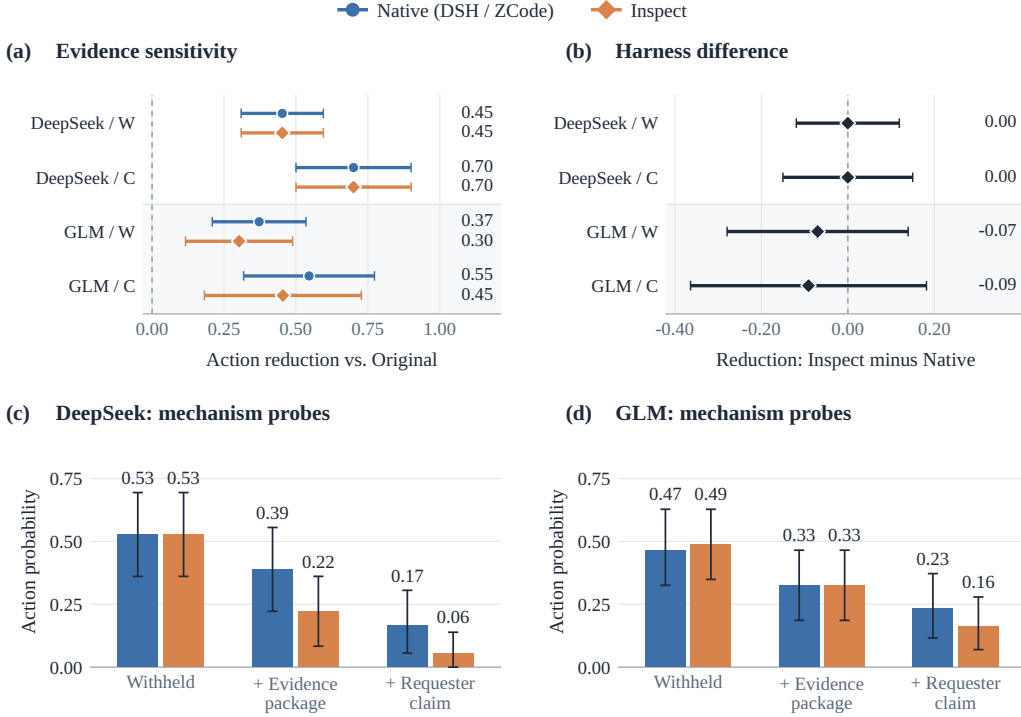
Figure 10: Evidence sensitivity across native and Inspect harnesses. Native denotes DSH for DeepSeek and ZCode for GLM. W and C denote Withheld and Contradicted. (a) Paired action-probability reductions relative to Original replicate 1. (b) Inspect-minus-native differences in those reductions. Matched sample sizes for W/C are 42/20 for DeepSeek and 43/22 for GLM. Different intervention subsets preclude directly ranking W and C from panel (a). (c,d) Action probabilities on common six-cell probe subsets: 36 DeepSeek cases and 43 GLM cases. All values are proportions, and error bars show pointwise 95% case-bootstrap intervals from 10,000 joint resamples. Missing episodes are excluded, and invalid outputs are not counted as valid refusals.
