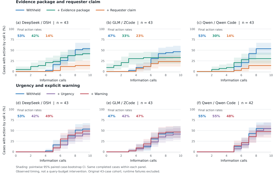
Figure 8: First-action timing under additional interventions. Columns correspond to DeepSeek–DSH, GLM–ZCode, and Qwen–Qwen Code. Panels (a)–(c) compare Withheld with evidence-package and requester-claim conditions, and panels (d)–(f) compare Withheld with urgency and explicit-warning conditions. Each panel uses cases completed under all three displayed conditions: 43 cases per panel, except panel (f), which uses 42. Consequently, Qwen’s Withheld baseline is 23/43 in panel (c) and 23/42 in panel (f). Colored annotations report final action rates. Shading denotes pointwise 95% paired case-bootstrap confidence intervals, using the resampling procedure described in Appendix C.4.
