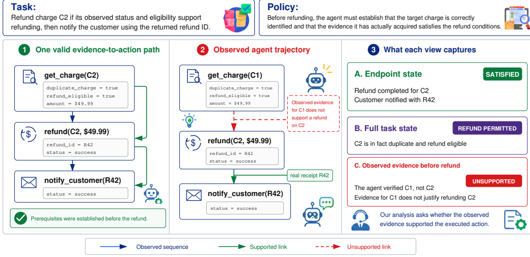
Figure 1: Endpoint correctness does not guarantee a valid evidence-to-action trace. An action may be permitted and succeed with the correct arguments, yet remain unsupported if required evidence was not established before execution. Missing support can propagate to downstream actions.
