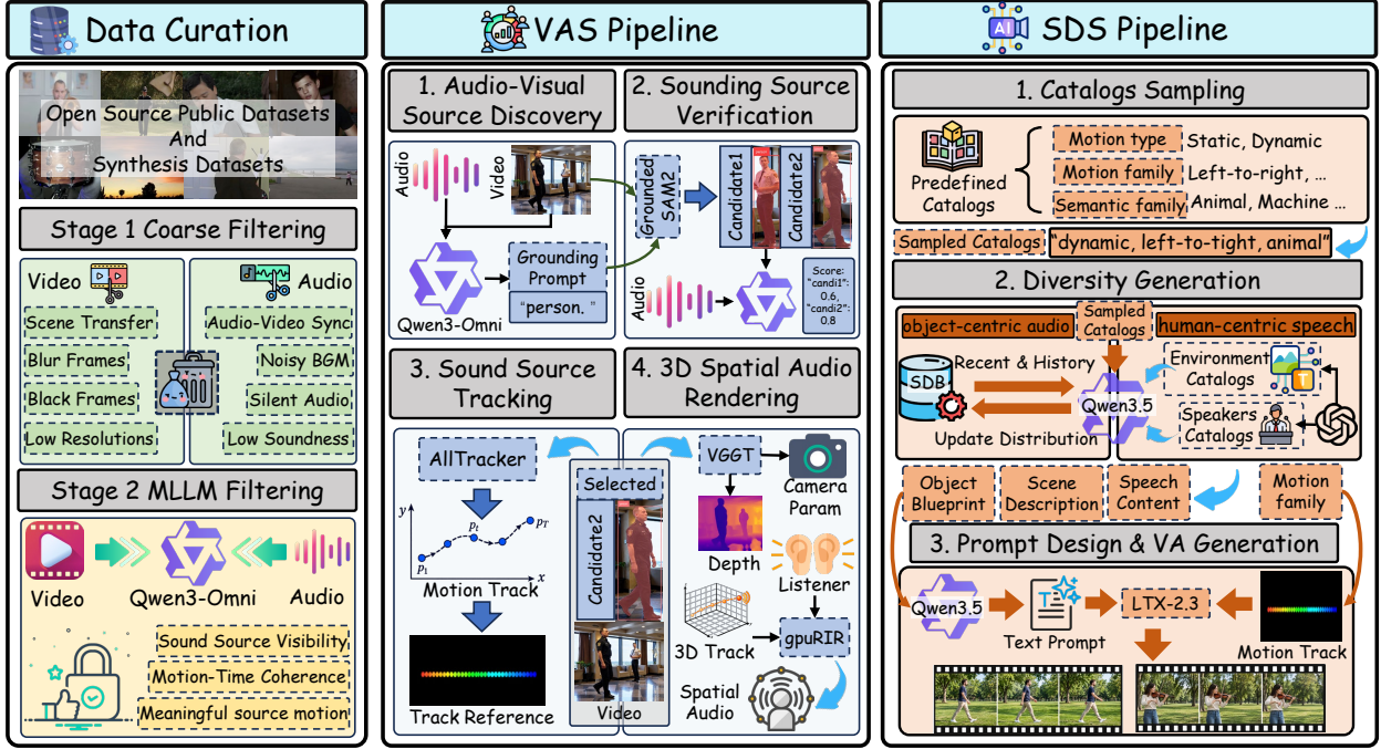
Figure 2 Construction pipeline of StereoWorld-29K. We combine curated real-world videos with synthetic audiovisual data. The VAS Pipeline localizes and tracks sound sources and renders track-guided stereo audio, while the SDS Pipeline generates diverse track-controlled scenes.
