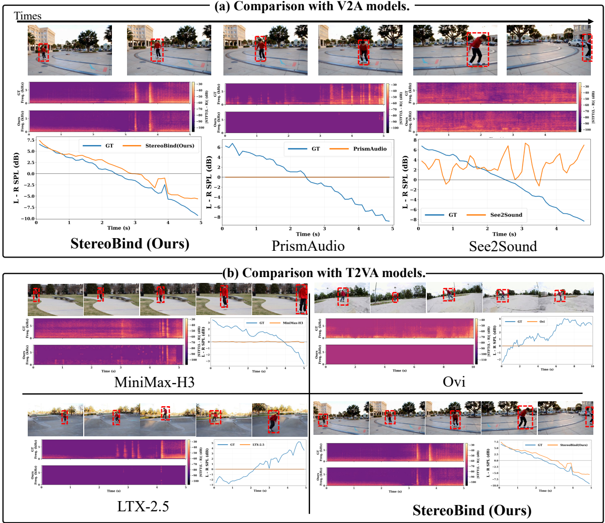
Figure 4 Qualitative experimental results on SWBench. We compare StereoBind with open-source VA models and V2SA models. The sound source is highlighted with a red bounding box.
