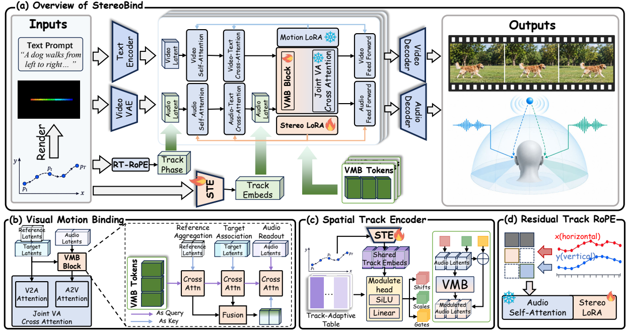
Figure 3 Overview of the StereoBind framework. StereoBind introduces VMB for audiovisual source binding, STE for absolute track conditioning, and RT-RoPE for relative motion modeling.
