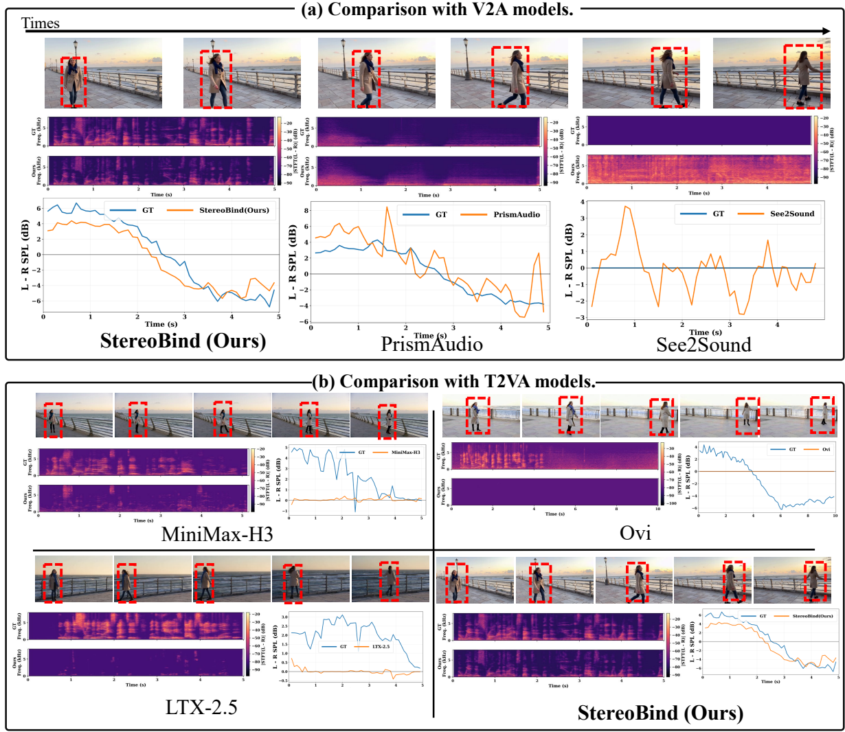
Figure 9 Qualitative experimental results on SWBench. We compare StereoBind with open-source VA models and V2SA models. The sound source is highlighted with a red bounding box.
