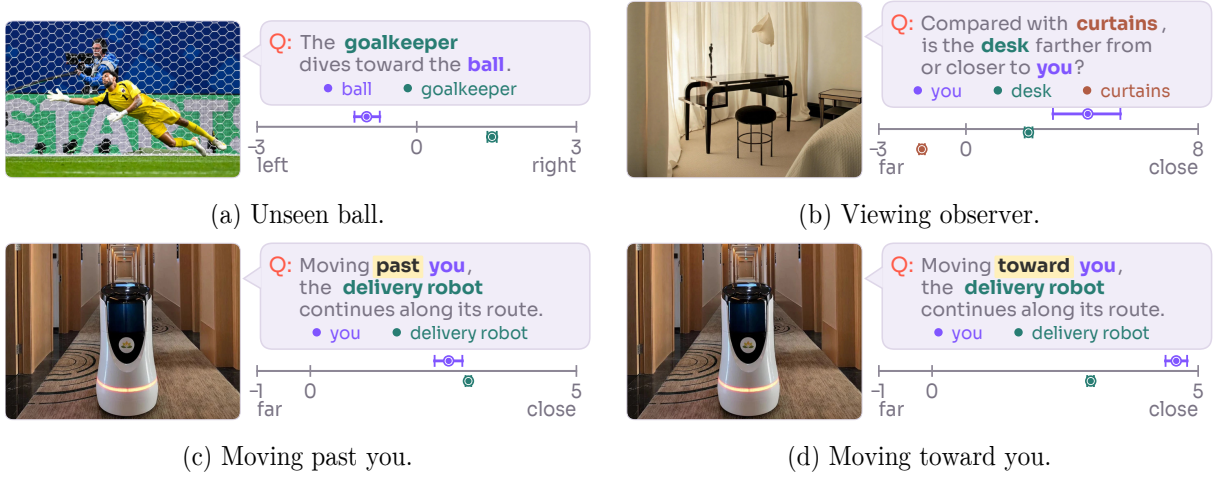
Figure 6 S-Space beyond visible objects. It localizes off-screen entities (a), places the invisible observer (b), and reflects relations implied by language (c-d). Readout from Molmo2-ER L17. Bars show 95% prompt-template bootstrap intervals.
