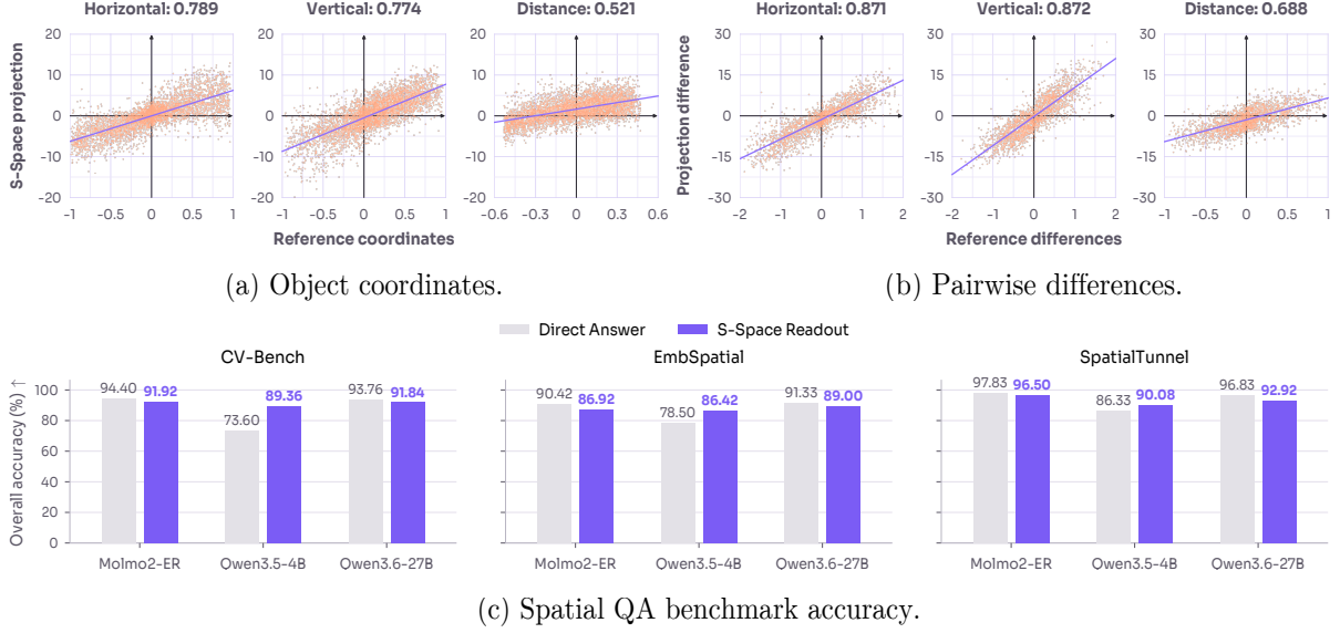
Figure 3 Accuracy of S-Space. (a-b) S-Space coordinates read from layer 21 of Molmo2-ER versus ground-truth object positions, with Spearman correlations and least-squares fits. (c) Spatial QA accuracy across benchmarks and models, comparing S-Space readouts with models’ direct answers.
