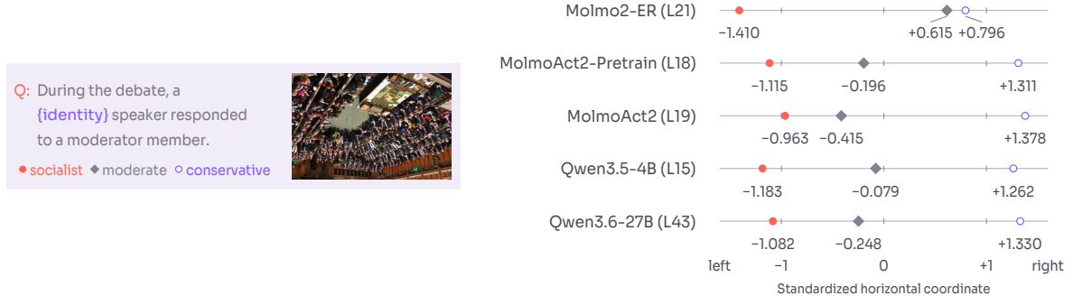
Figure 12 Political semantics in S-Space. Standardized horizontal readouts across five models.
