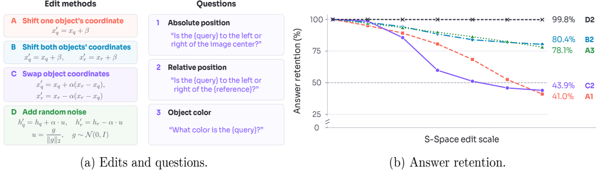
Figure 4 Causal intervention of S-Space. (a) Different coordinate-editing and question configurations. (b) Answer retention under different interventions and edit scales. Experiments use Molmo2-ER at layer 17 (L17). See Appendix C.3 for details.
