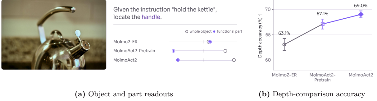
Figure 14 Action training sharpens part-whole depth geometry in S-Space. (a) Depth readouts for the kettle and its handle. (b) Depth comparison accuracy at L18 for all three models. Error bars indicate 95% confidence intervals across prompts.
