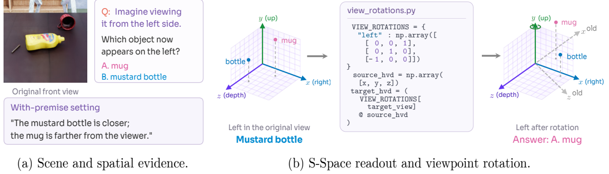
Figure 8 Perception-Computation decomposition via S-Space. (a) Perspective-taking question and the optional w/ premise setting. (b) We separate spatial perception from spatial computation by reading object coordinates from S-Space, applying the viewpoint transformation explicitly, and deriving the answer with a deterministic spatial rule.
