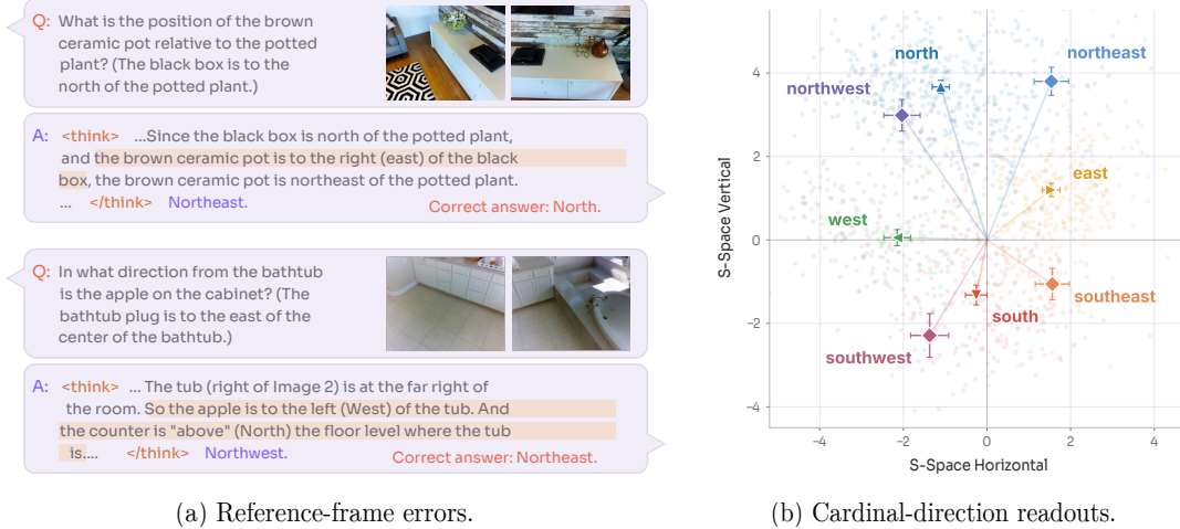
Figure 10 Direction coupling in S-Space. (a) Representative reasoning failures where image-relative relations are incorrectly reused as cardinal directions. (b) S-Space coordinates of cardinal-direction tokens from Qwen3.6-27B chain-of-thought on MMSI-Bench.
