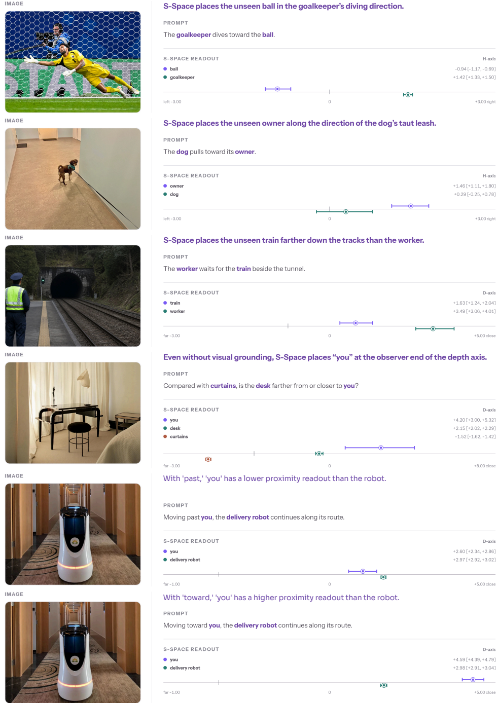
Figure 11 S-Space beyond visible objects. Images, prompts, and horizontal or distance readouts for an unseen ball, owner, train, the observer, and a robot moving past or toward. Readouts use Molmo2-ER L17. Means and 95% bootstrap intervals are computed across prompt templates.
