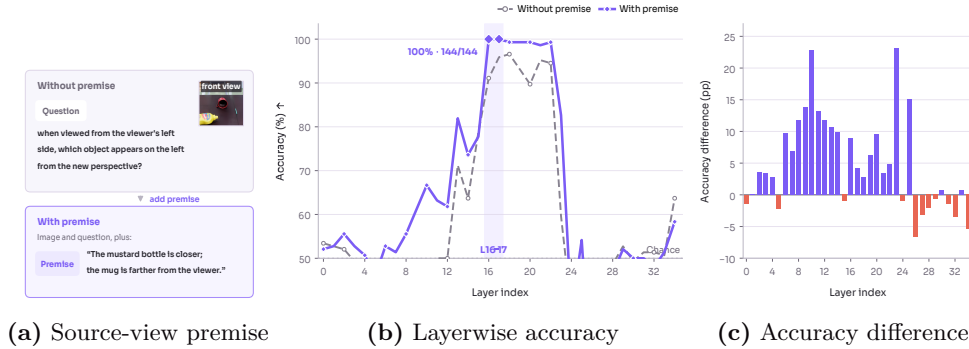
Figure 13 Molmo2-ER readouts with spatial premises. (a) Source-view premise. (b) Layerwise accuracy with ( n = 144 ) and without ( n = 146 ) premises. (c) Accuracy difference.
