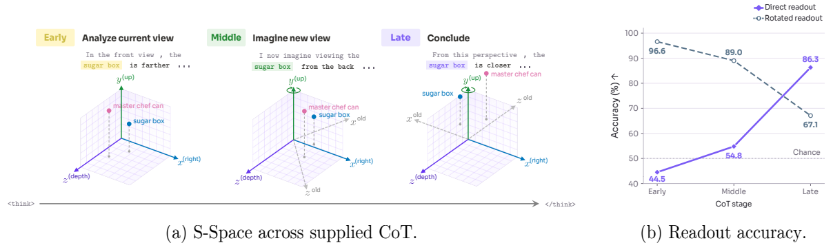
Figure 9 Chain-of-thought progressively transforms S-Space. (a) S-Space coordinates read out from object names at successive stages of a controlled CoT. (b) Qwen3.6-27B L43 readout accuracy on SpinBench with and without explicit viewpoint rotation.
