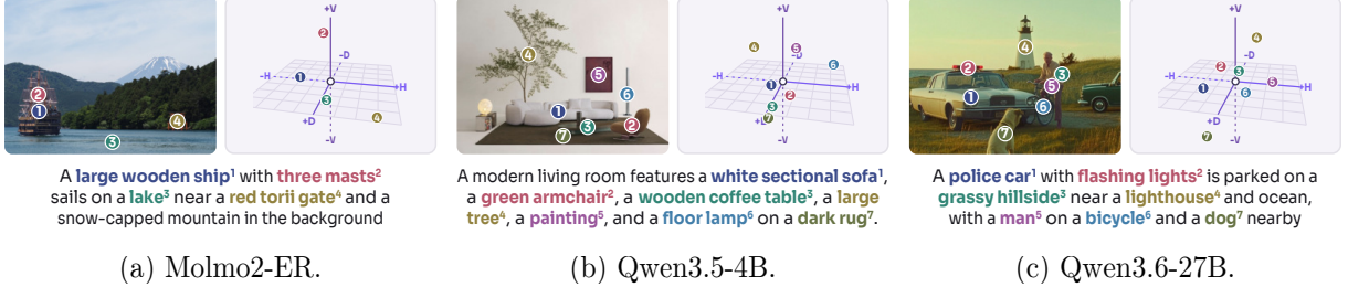
Figure 1 Object coordinates read out from S-Space across MLLMs. For each input image and caption, the intermediate representations of object-name tokens are linearly projected onto the three axes of S-Space to obtain continuous coordinates. Colors and numbers link object names, image regions, and their corresponding coordinates.
