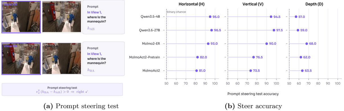
Figure 15 Prompt steering test of S-Space in multi-view contexts. (a) Each example is evaluated twice with the same View-1 query while the two input images are swapped. (b) We evaluate the sign agreement between the resulting change in the S-Space coordinates and the object’s ground-truth displacement between the two views.
