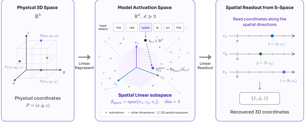
Figure 2 Linear spatial representation in S-Space. An object’s spatial coordinates ( left ) are linearly embedded in its high-dimensional token representation. Horizontal, vertical, and distance directions span a three-dimensional S-Space ( middle ). Projections onto them recover viewer-centered coordinates ( right ).
