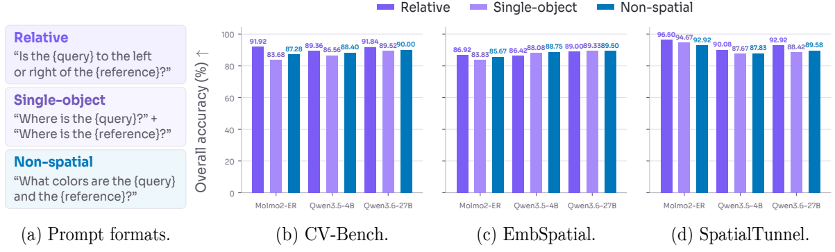
Figure 5 S-Space persists across prompts. The same S-Space readout continues to support accurate spatial judgments on CV-Bench, EmbSpatial, and SpatialTunnel (b-d) across pairwise spatial, single-object, and non-spatial prompts (a).
