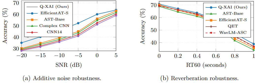
Figure 2: Robustness of Q-XAI under acoustic degradation. Left: accuracy vs. SNR under additive white noise. Right: accuracy vs. RT60 under simulated reverberation. Q-XAI degrades more gracefully than all baselines in both conditions.
