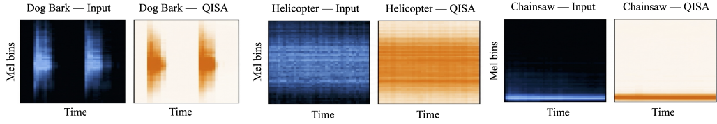
Figure A2: Additional QISA attribution maps for ESC-50 categories (schematic heatmaps; brighter = higher attribution). Dog Bark : temporal bursts dominate at mid frequencies; QISA correctly ignores the silent inter-burst intervals. Helicopter : broadband persistent energy across all frames; QISA attributes uniformly to the continuous rotor signature. Chainsaw : concentration at the lowest mel band reflects the persistent low-frequency two-stroke harmonic, the most discriminative cue.
