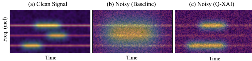
Figure 3: QISA attribution maps for a “street traffic” scene (schematic heatmaps; brighter = higher attribution). (a) Clean signal: attribution concentrates on harmonic frequency bands (rows 2 and 4), corresponding to engine-idling fundamentals. (b) Heavy noise (−5 dB SNR), real-valued model: attribution diffuses uniformly across the spectrogram, losing discriminative structure. (c) Heavy noise, Q-XAI: phase-selective attention preserves the harmonic band structure, focusing on phase-coherent components that survive under noise.
