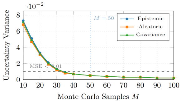
Figure 4: AUQ convergence: variance of all three uncertainty components as a function of Monte Carlo samples M on DCASE 2019 ( n = 10 runs). All components stabilise below \text{MSE} = 0.01 at M = 35 ; M = 50 is chosen as a conservative operating point.
