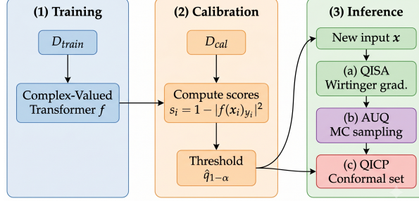
Figure 1: Q-XAI framework overview. (1) Training: the CVT is trained on \mathcal{D}_{\text{train}} . (2) Calibration: nonconformity scores are computed on a held-out set \mathcal{D}_{\text{cal}} to determine the QICP threshold \hat{q}_{1-\alpha} . (3) Interpretable inference: for a new input, Q-XAI simultaneously produces (a) a QISA saliency map via Wirtinger backpropagation, (b) AUQ uncertainty estimates via Monte Carlo sampling, and (c) a QICP prediction set with formal coverage guarantees.
